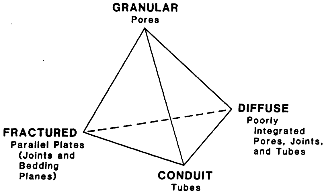
Figure 1. Relation between four major types of aquifers and the dominant porosity geometry in each. This is a tetrahedral continuum. (after Quinlan & Ewers, 1985)
